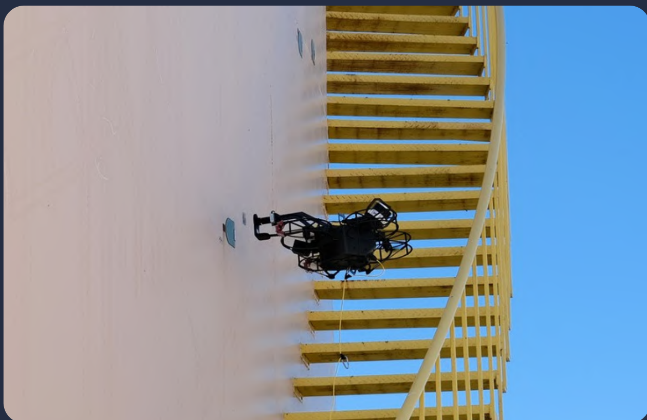
Figure 5: Example of WAND-PDC data collection using the ScoutDI 137 Gen 3
