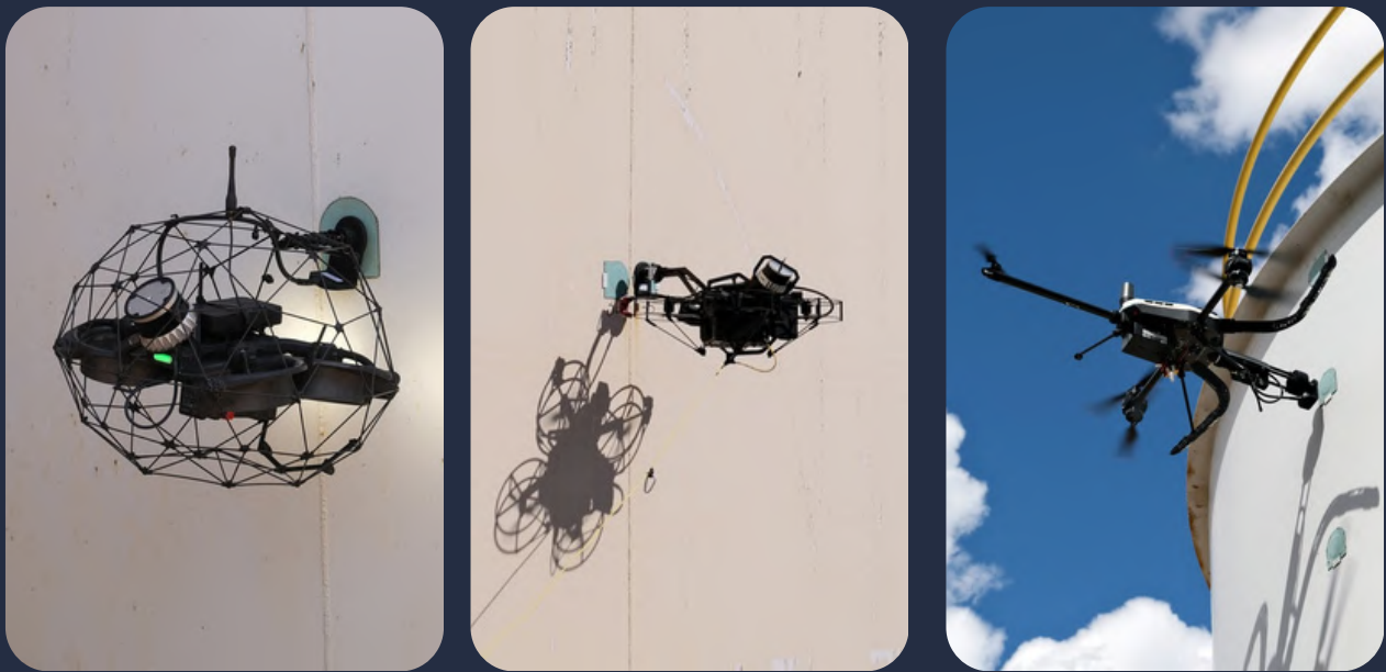
Figure 1: Sensor locations and drone-enabled data collection from tank assets
