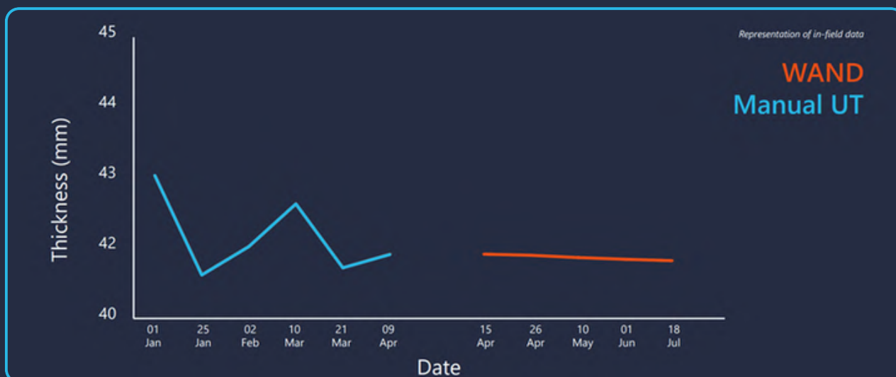
Figure 6: Transition from manual UT measurements to the WAND solution
